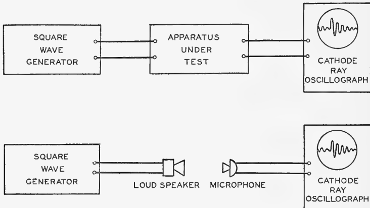
FIG. 11.14. — Schematic arrangement of the apparatus employing a square wave generator and a cathode ray tube for indicating the transient response characteristics of acoustical apparatus such as microphones or loud speakers.
